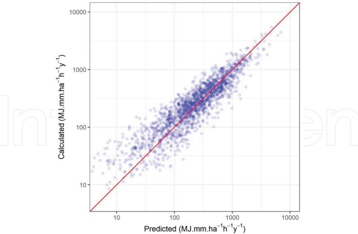
Figure 8. Calculated annual erosivity values coming from pluviograph data versus predicted values using the neural network on the testing set. With red line, the identity function f(x) = x is symbolized.
